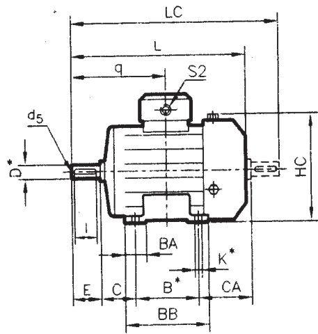
FRAME SIZE 63, 71 & 80
