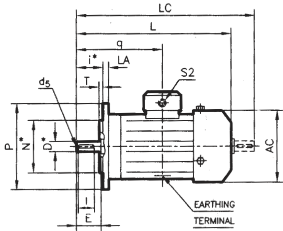
FRAME SIZE 63, 71 & 80
